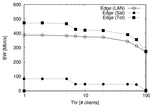
Fig. 3: Bandwidth utilization
